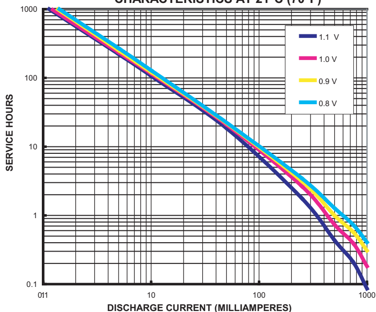
TYPICAL DISCHARGE CHARACTERISTICS AT 21°C (70°F)
